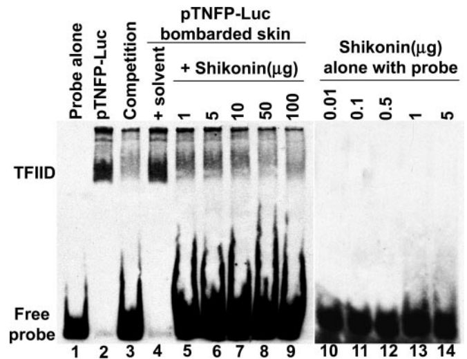
FIG. 9. Shikonin inhibits the TFIID complex (TBP) binding to TATA box in TNF- \alpha promoter. Mouse skin was bombarded with pTNF-Luc DNA-coated gold particles and either untreated or treated with solvent alone or shikonin at different concentrations. Skin samples were harvested after 1 h, and nuclear extracts were subjected to EMSA as described under "Experimental Procedures" (lanes 2 and 4–9). Binding specificity of the complexes was analyzed with 200-fold excess of unlabeled DNA probe competition (lane 3). Direct binding of shikonin to the probe was tested by incubating different concentrations of shikonin with the labeled probe (lanes 10–14).
