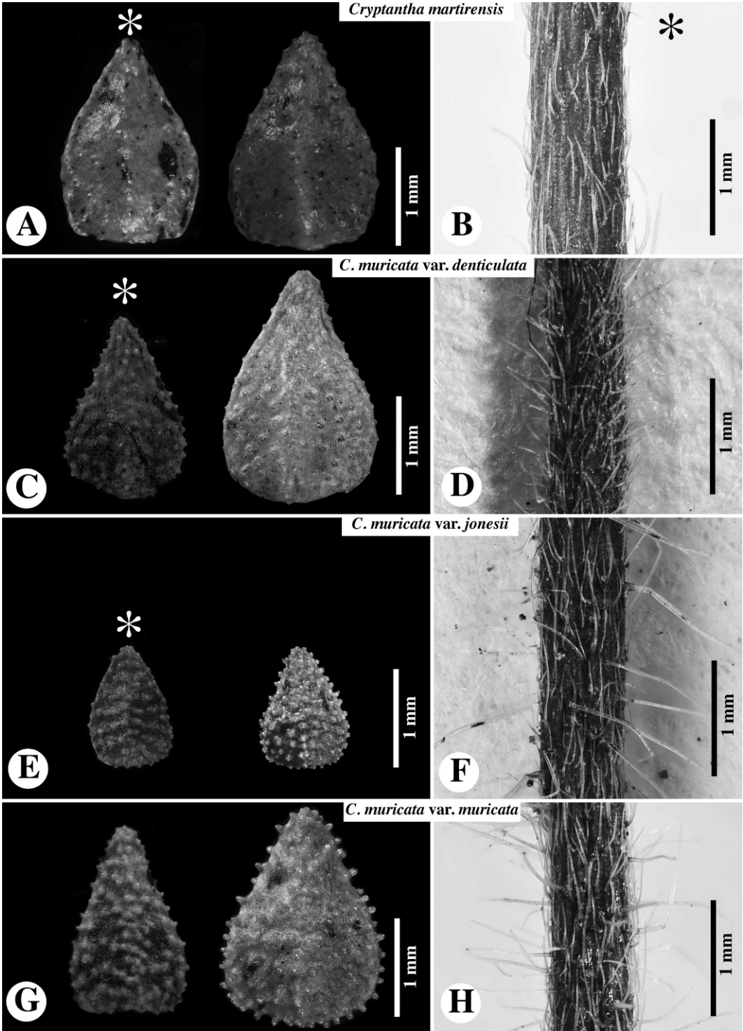
FIG. 6. Comparisons of nutlets and inflorescence axis of investigated taxa. A–B. Cryptantha martirensis . A. Nutlets (left = Rebman 15993 ; right = Rebman 15973 ). B. Inflorescence axis ( Rebman 15993 ). C–D. Cryptantha muricata var. denticulata . C. Nutlets (left = Curran s.n. , CAS 123277; right = Simpson 2910 ). D. Inflorescence axis ( DeDecker 3354 ). E–F. Cryptantha muricata var. jonesii . E. Nutlets (left = Jones 79 [GH 97680]; right = Howe 996 ).
