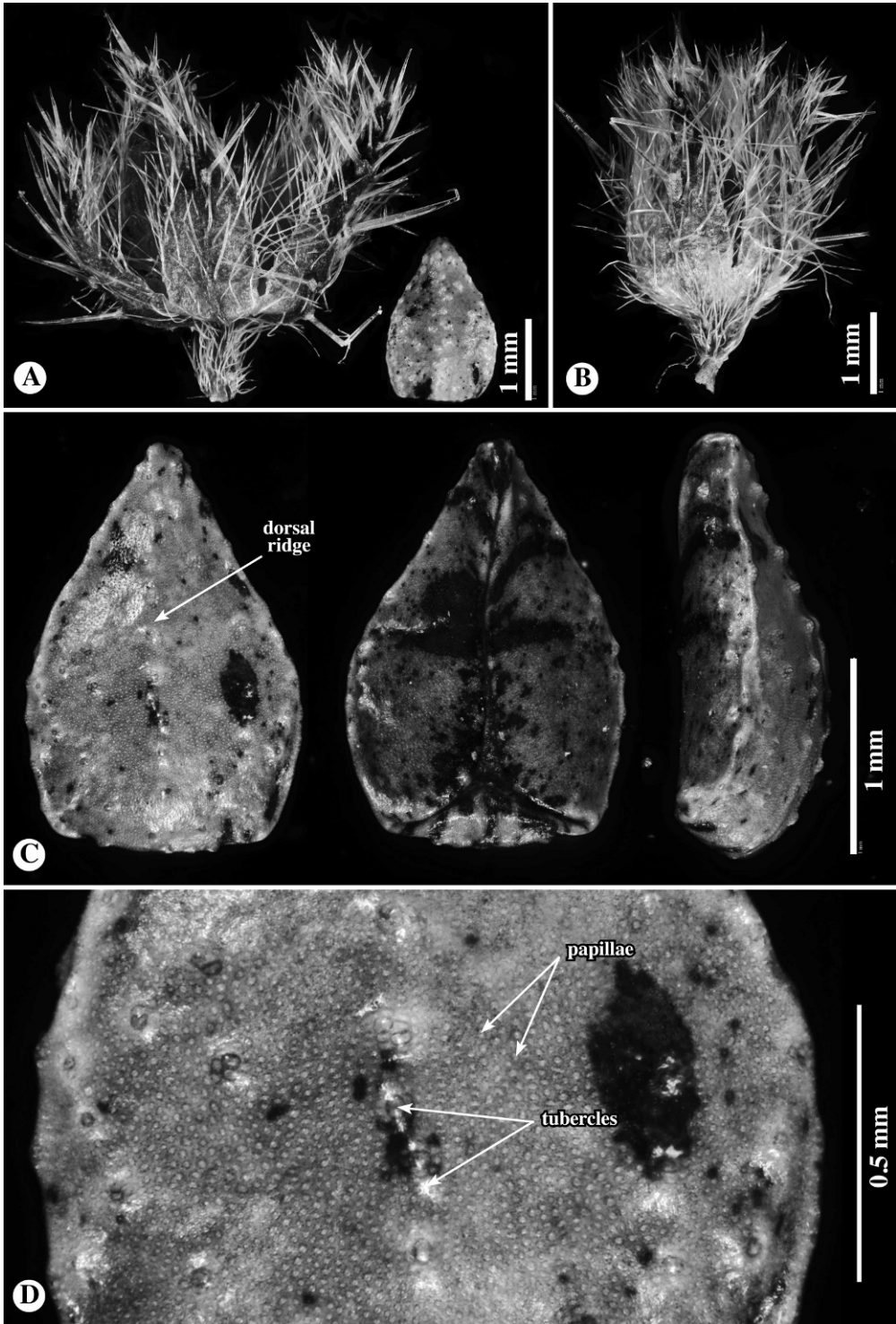
FIG. 3. Cryptantha martirensis . A. Calyx in fruit, with one of four nutlets ( Rebman 16022 ). B–D. ( Rebman 15993 , type specimen). B. Calyx in fruit. C. Nutlet, in dorsal (left), ventral (middle) and lateral (right) views. Note dorsal ridge. D. Nutlet dorsal surface, close-up. Note numerous papillae and low tubercles.
